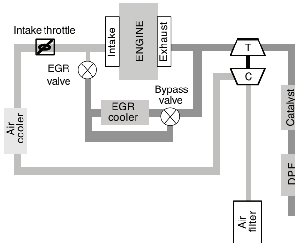
Figure 7 Engine architecture.
