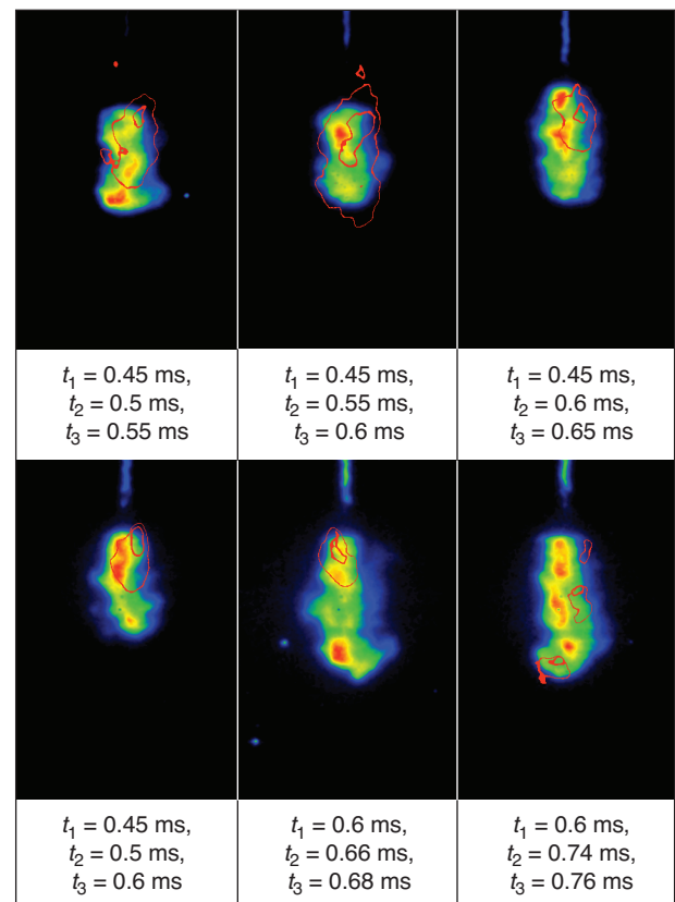
Figure 13 Processed images of LIF and contours of auto-ignition sites. P_{inj} = 1000 bar, image size 34 \times 54 mm 2 .
