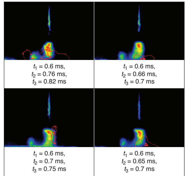
Figure 20 Processed images of LIF and contours of auto-ignition sites. P_{inj} = 1000 bar, d_{nw} = 2.5 cm, image size 50 \times 27 mm 2 .
