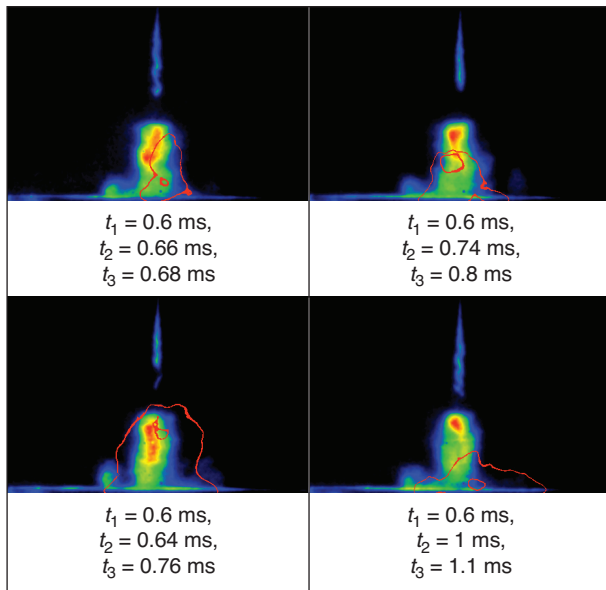
Figure 18 Processed images of LIF and contours of auto-ignition sites. P_{inj} = 1000 bar, d_{nw} = 3.5 cm, image size 50 \times 31.5 mm 2 .
