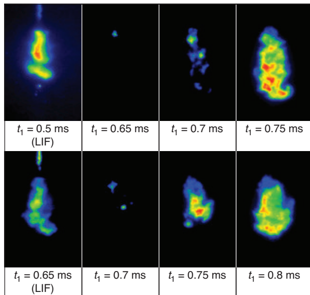
Figure 14 Two time sequences of LIF and direct visualizations of combustion realized with the high speed camera. P_{inj} = 1500 bar, image size 30 \times 45 mm 2 , time between images 50 \mu\text{s} .
