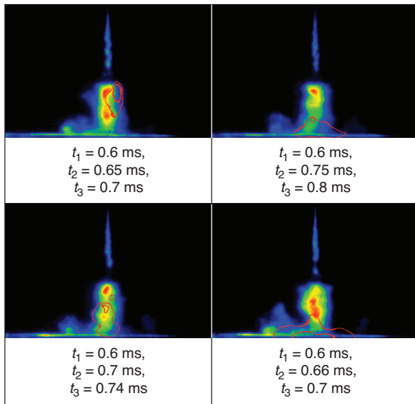
Figure 19 Processed images of LIF and contours of auto-ignition sites. P_{inj} = 1400 bar, d_{nw} = 3.5 cm, image size 50 \times 31.5 mm 2 .
