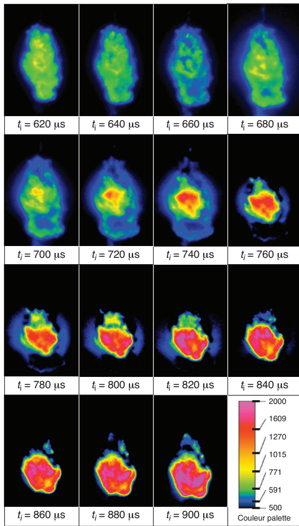
Figure 12 Time sequence of direct visualizations of combustion realized in the same event with the high speed camera. P_{inj} = 1000 bar, image size 30 \times 45 mm, time between images 20 \mu\text{s} .
