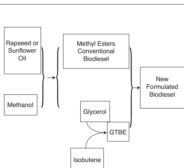
Figure 6 New biodiesel formulation.
