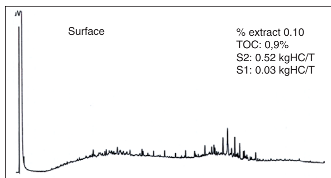
Chromatogram of saturated hydrocarbons
