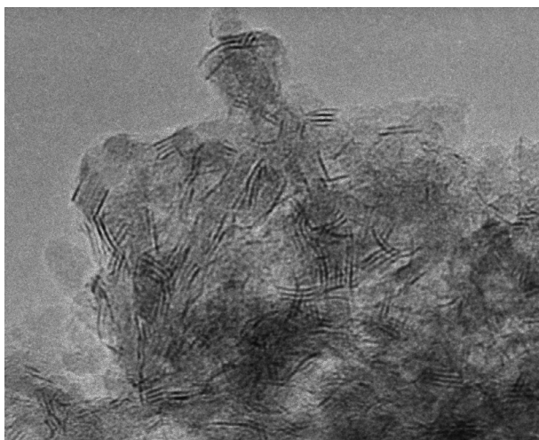
Figure 10 Transmission electron microscopy micrograph of the CoMoP(0.5)-S catalyst.
