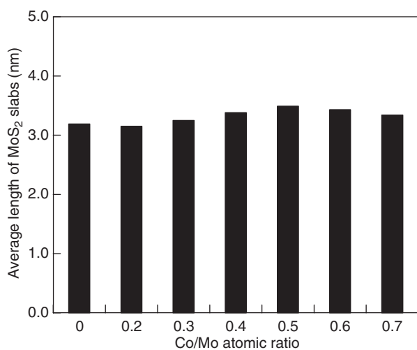
Figure 12 Average length of MoS 2 slabs determined by TEM, for the sulfided CoMoP catalysts at various Co/Mo ratios.
