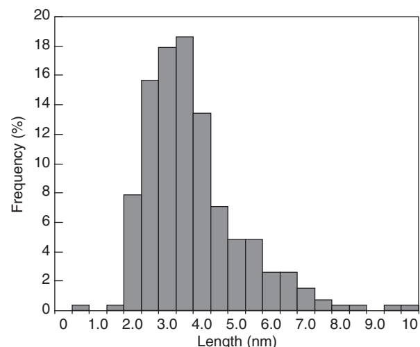
Figure 11 Histogram of the length of MoS 2 slabs realized from the analysis of the CoMoP(0.5)-S by TEM.
