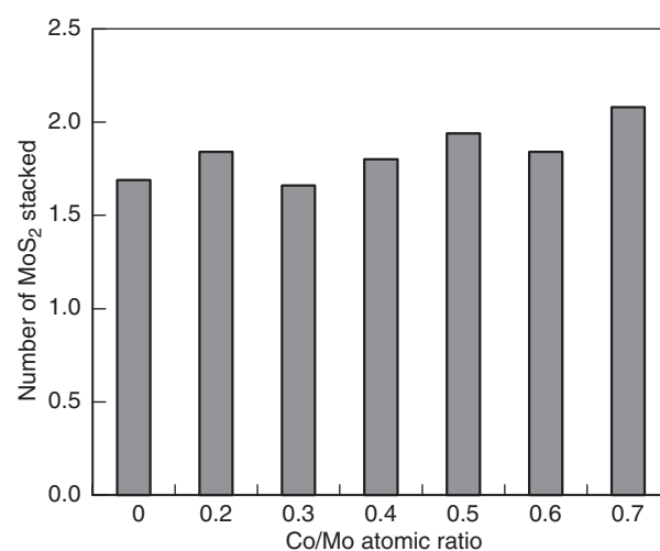
Figure 13 Average number of stacked MoS 2 slabs determined by TEM, for the sulfided CoMoP catalysts at various Co/Mo ratios.
