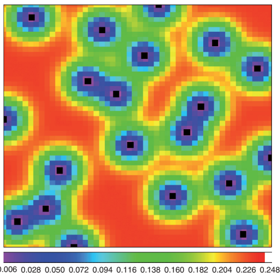
Figure 6 Kriging variance.
