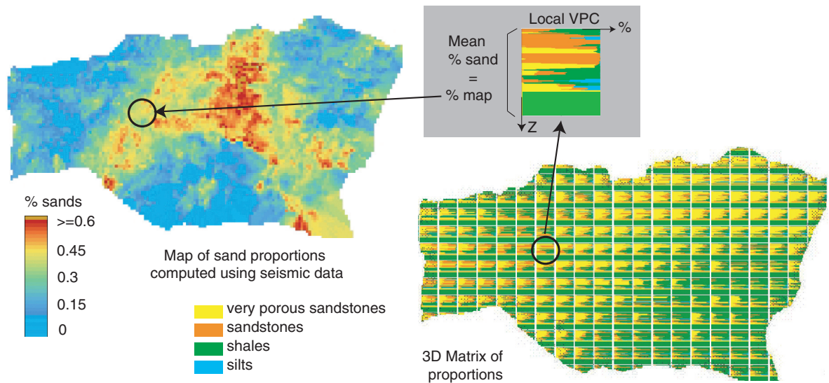
Figure 5 3D matrix of proportions computed using a map of trend of proportions.
