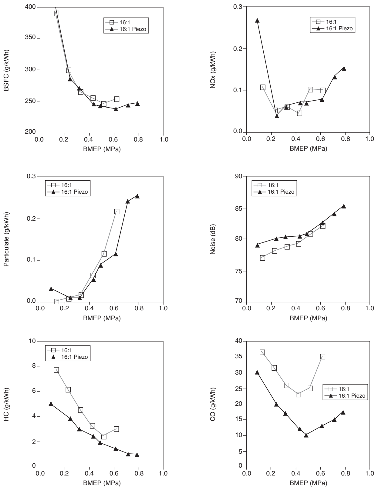
Figure 10 Injection system effect on engine results, 1500 rpm.
