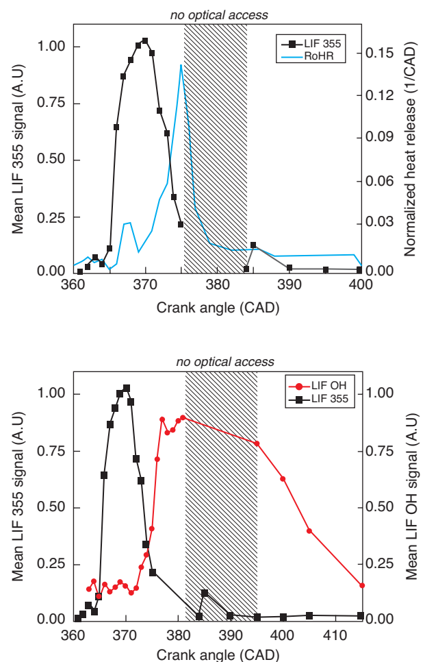
Figure 17 Comparison of the temporal evolution of the mean LIF 355 signal relative to the heat release rate (upper graph) and mean LIF OH signal (lower graph) for the bowl-dome piston geometry.
