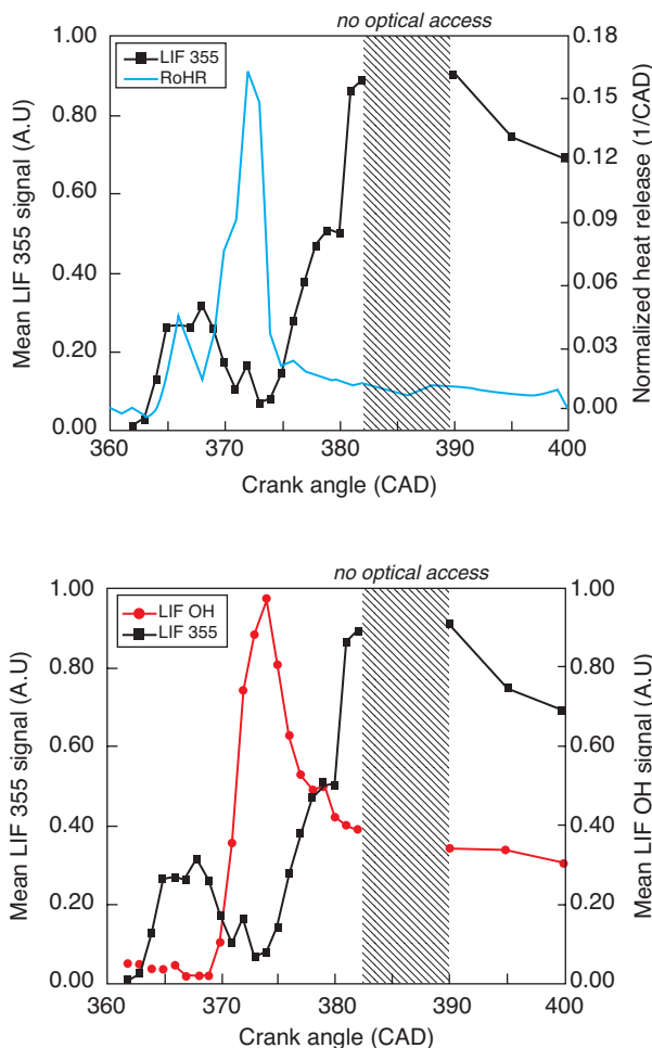
Figure 16 Comparison of the temporal evolution of the mean LIF 355 signal relative to the heat release rate (upper graph) and mean LIF OH signal (lower graph) for the flat piston geometry.
