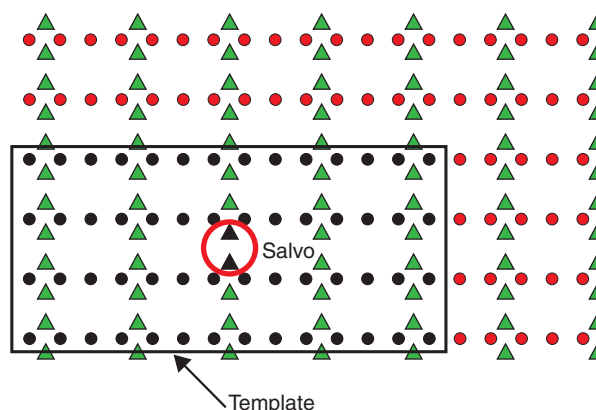
Figure 10 Salvo: shot points within the red circle. Black rectangle defines the template.
