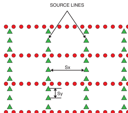
Figure 9 Source ligne: a line where source points are located at a regular distance. Receiver lines: horizontal lines. Source lines: vertical lines.
