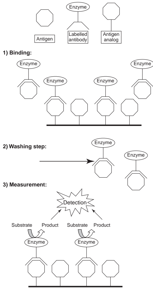
Figure 10 Competitive immunoassay.
