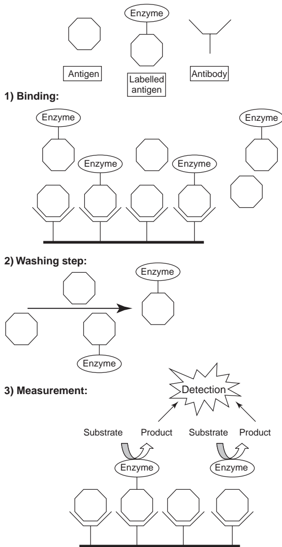
Figure 9 Competitive immunoassay.
