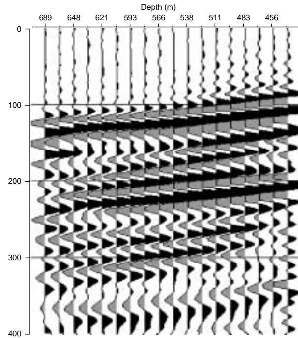
Figure 52 BHA1. Zw well component. Rig source collection. Figs 52, 53 and 54: isotropic 3C displays, filtered (2, 65 Hz). Constant gain. Observation: components XV and YH do not show a good trace to trace coherency.
