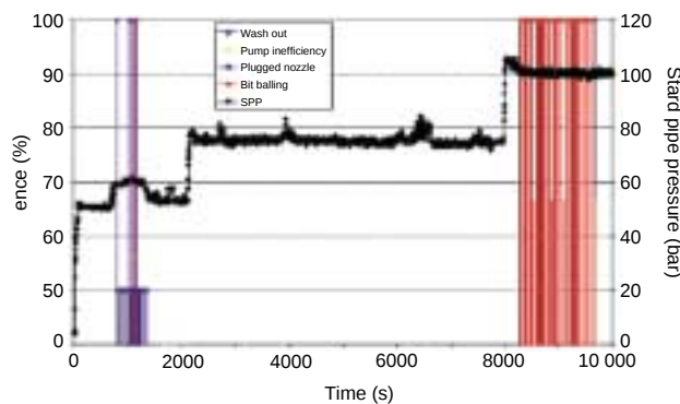
Figure 13 Field test of the system.
