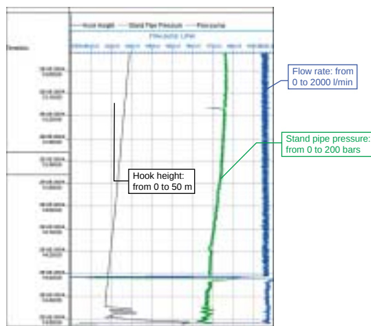
Figure 14 Display of a drill pipe wash out occurring at the well site.
