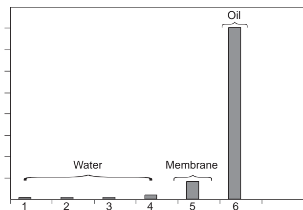
Figure 7 SEM/EDS observation – Encapsulated System A – Monomers 0.7 mol/l – C/O ratio evolution through the membrane.
