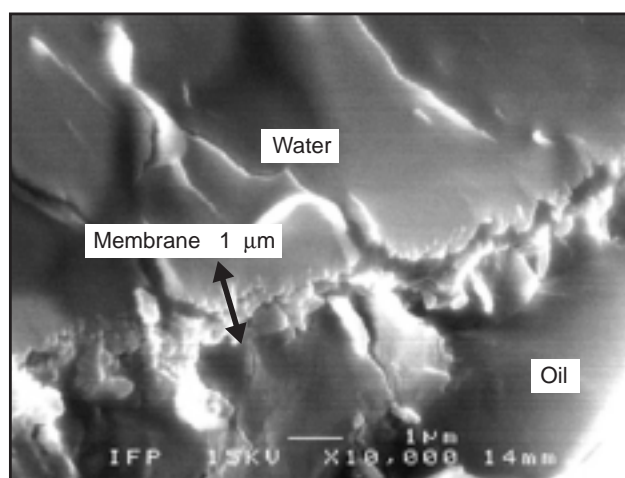
Figure 5 SEM observation – Encapsulated System A – Monomers 0.7 mol/l.
