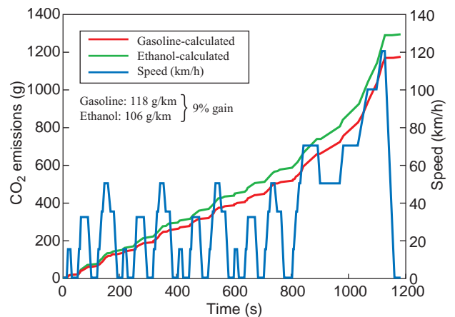
Figure 10 Calculation of CO 2 emissions on the NEDEC cycle.
