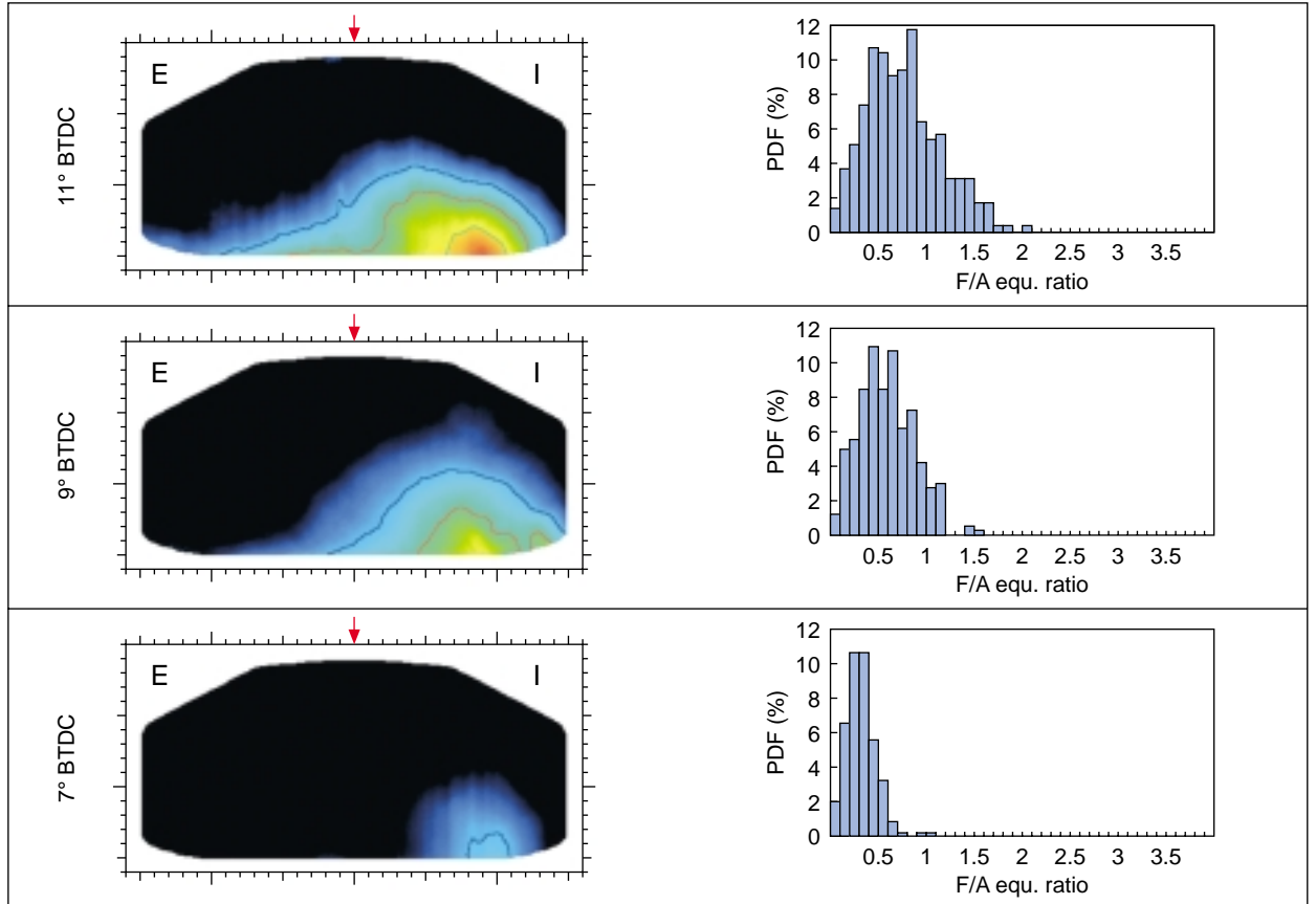
Figure 18 Mean fuel/air equ. ratio map and histogram in the ignition zone in condition C (early injection).
