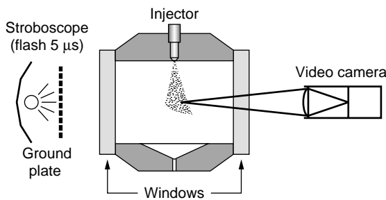
Figure 7 Spray imaging set-up.
