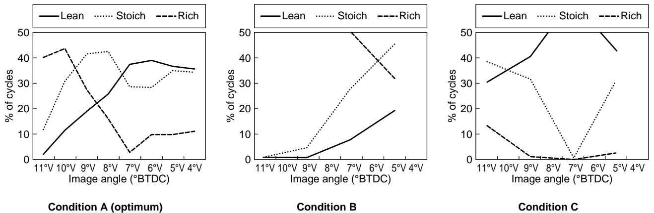
Figure 19 Percentage of cycles with lean, stoichiometric or rich conditions in the electrode gap versus crank angle.
