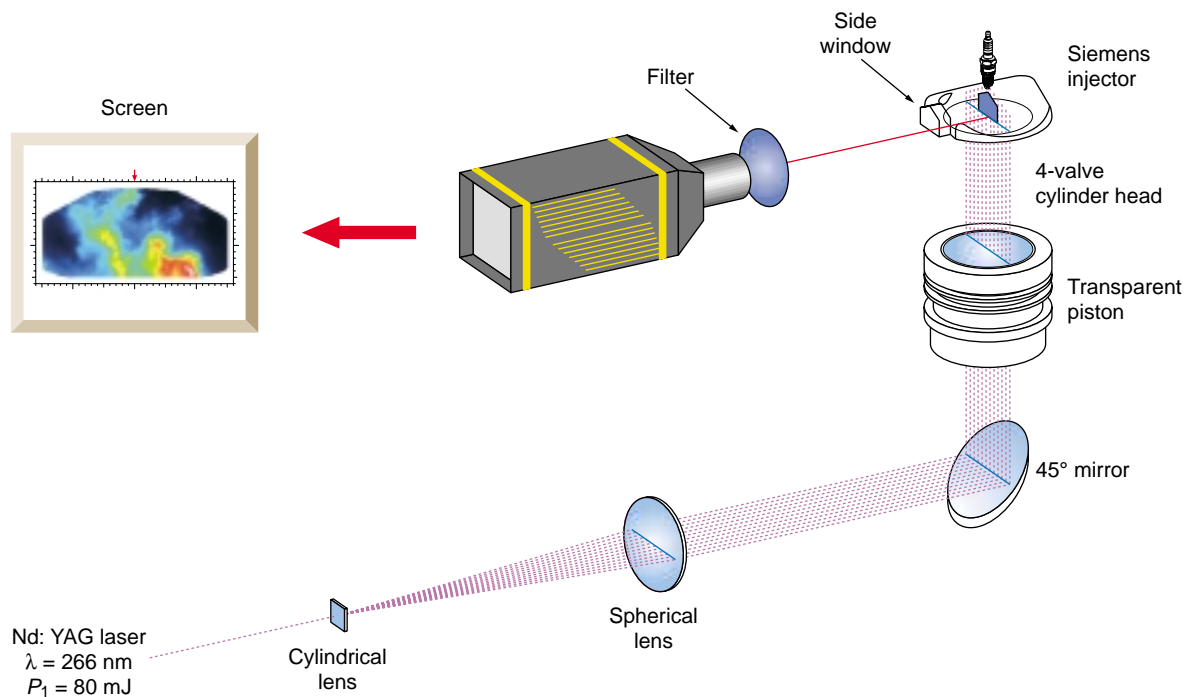
Figure 3 Laser-induced fluorescence arrangement.
