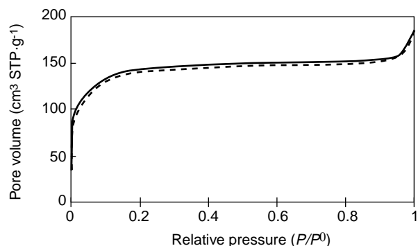
Figure 9 Nitrogen adsorption (—) and desorption (---) isotherms of the mesostructured alumina synthesized in the presence of sodium dodecyl sulfate and calcined at 450^\circ\text{C} .
