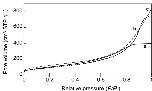
Figure 7 Nitrogen adsorption isotherms of samples synthesized by way B washed with water (a), ethanol (b), and acetone (c).
