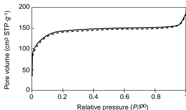
Figure 9 Nitrogen adsorption (—) and desorption (---) isotherms of the mesostructured alumina synthesized in the presence of sodium dodecyl sulfate and calcined at 450^\circ\text{C} .
