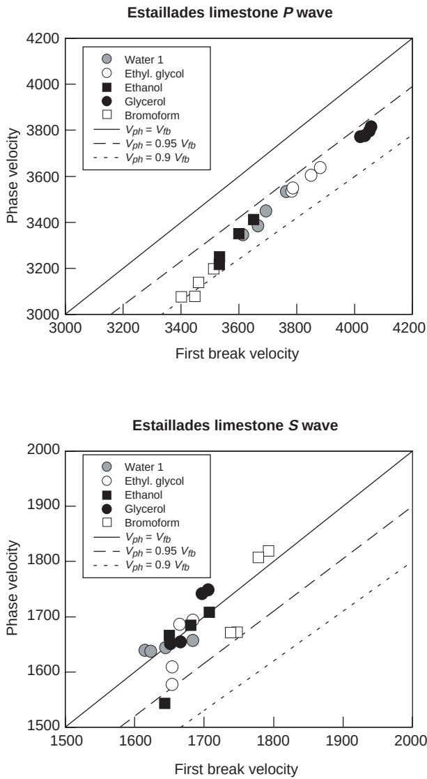
Figure 9 Comparison of phase velocities and first break picking velocities in Estailades limestone.
