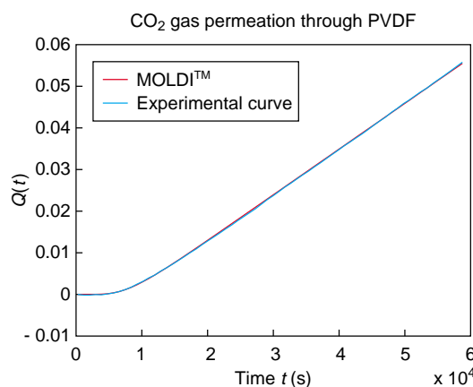
Figure 8 Flux Q (in moles per \text{cm}^2 ) of \text{CO}_2 through PVDF, as measured and calculated with MOLDI™.
