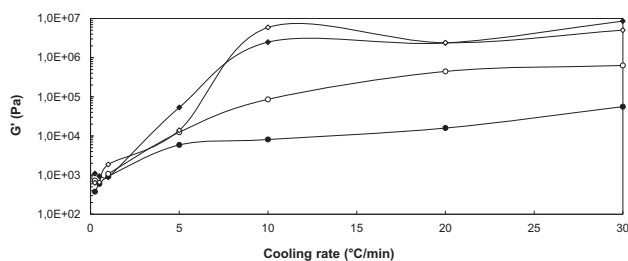
Fig. 11. Influence of cooling rate and holding time on the elastic modulus of crude oil S dynamically cooled under 50 \text{ s}^{-1} from 60 to 30 °C without any holding time after cooling ( \bullet ), with an holding time of 10 s ( \circ ), with an holding time of 2 min ( \blacklozenge ), and with an holding time of 3 h ( \diamond ).
