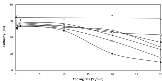
Fig. 12. Influence of cooling rate and holding time on the melting enthalpy of crude oil S cooled from 80 to 30 °C without any holding time after cooling ( \bullet ), with an holding time of 10 s ( \circ ), with an holding time of 30 s ( \blacktriangle ), with an holding time of 45 s ( \triangle ), with an holding time of 1 min ( \blacksquare ), with an holding time of 2 min ( \square ), and with an holding time of 5 min ( + ).
