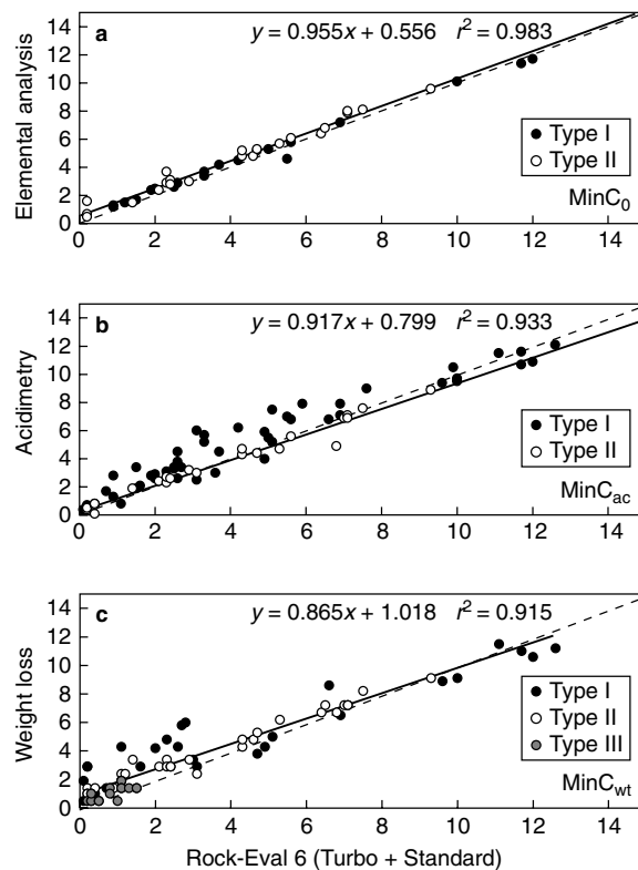
Figure 10 Correlation between Rock-Eval 6 (average values between Standard Rock-Eval 6 and Turbo Rock-Eval 6) obtained on source rocks for: (a) MinC and (TC - C_0) determined by elemental analysis for all data; (b) MinC and MinC determined by acidimetry; (c) MinC and the weight loss during decarbonation.
