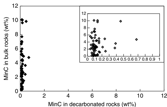
Figure 9 MinC values obtained by Rock-Eval 6 on decarbonated rocks.
