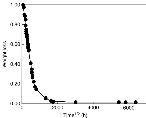
Figure 3 \text{CO}_2 desorption curve in LDPE at 22^\circ\text{C} .
