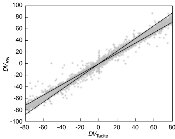
Figure 5 The difference DV between gas velocity and liquid velocity estimated by the neural networks system as function of DV given by Tacite.
