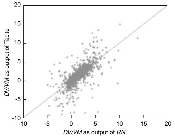
Figure 6 The ratio between the difference DV between gas velocity and liquid velocity estimated by the neural network system and the barycentric mixture velocity, V_M , as function of the same ratio given by Tacite.
