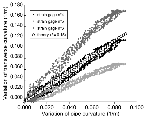
Figure 18 Theoretical and measured transverse curvatures at neutral bending axis.
