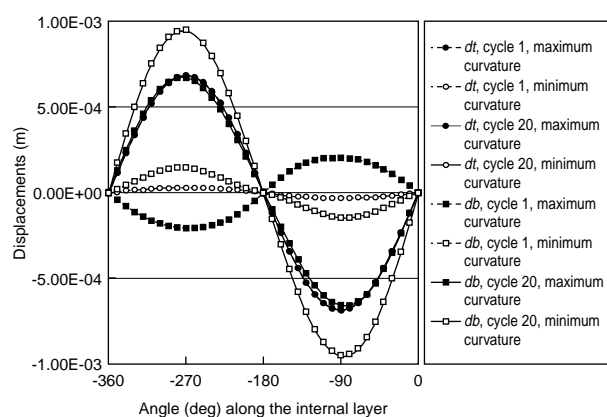
Figure 7 Displacements \Delta_i and \Delta_b along the internal armour layer.
