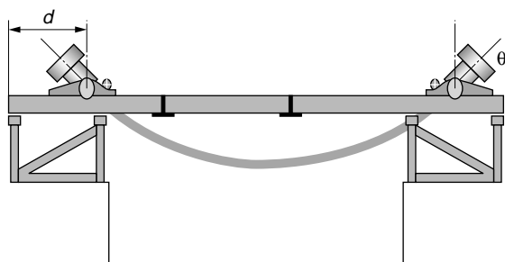
Figure 15 Dynamic bench test.
