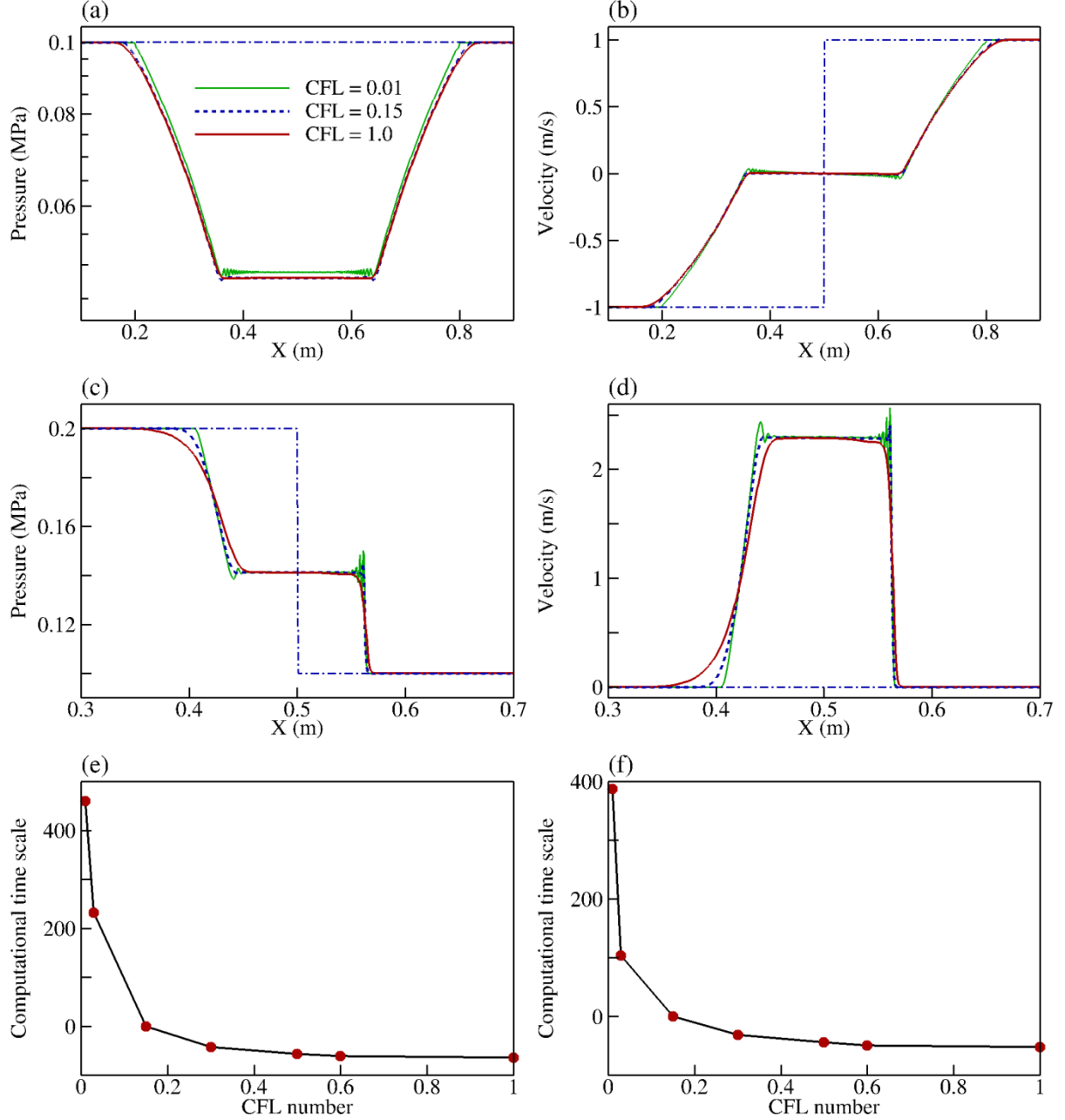
Fig. 9 Time-step analysis (CFL number) for Case 2 (a, b, e, t = 3.5 ms) and Case 4 (c, d, f, t = 2.0 ms), \varepsilon_{UVn} = 1.0\text{e-}13 , computational time scale = 100 \times (t_{CFL} - t_{CFL=0.15})/t_{CFL=0.15}
