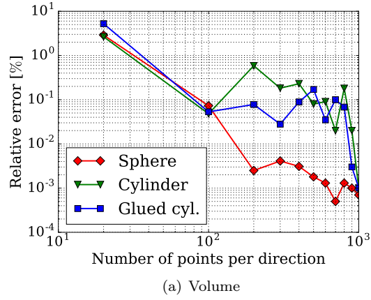
Figure 3 Relative error on (a) the volume and (b) components of the moment of inertia tensor, of a sphere, a cylinder and a glued convex made of two overlapping cylinders, as a function of the number of discretization points per direction.
