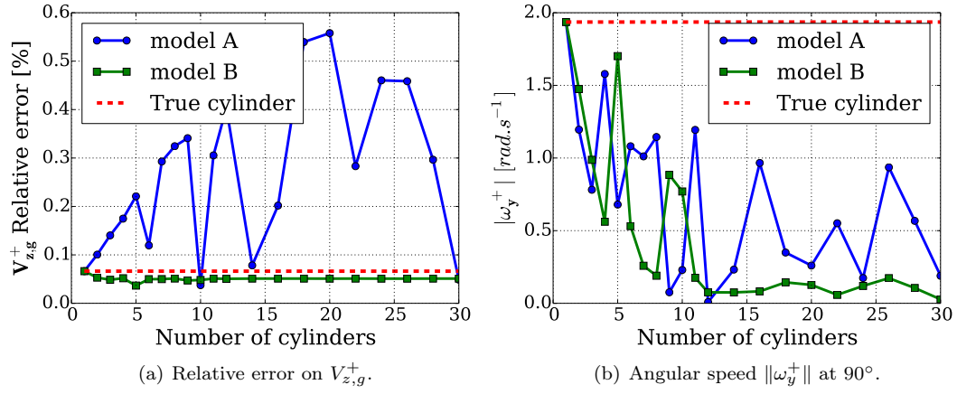
Figure 9 Cylinder-wall impact test case at an angle of 90°: error on post-impact velocities to the analytical solution for a true cylinder and for the 2 models as a function of the number of elementary cylinders of the glued cylinder .
