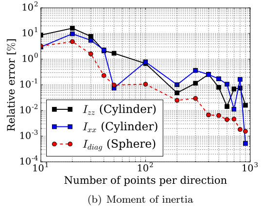
Figure 3 Relative error on (a) the volume and (b) components of the moment of inertia tensor, of a sphere, a cylinder and a glued convex made of two overlapping cylinders, as a function of the number of discretization points per direction.
