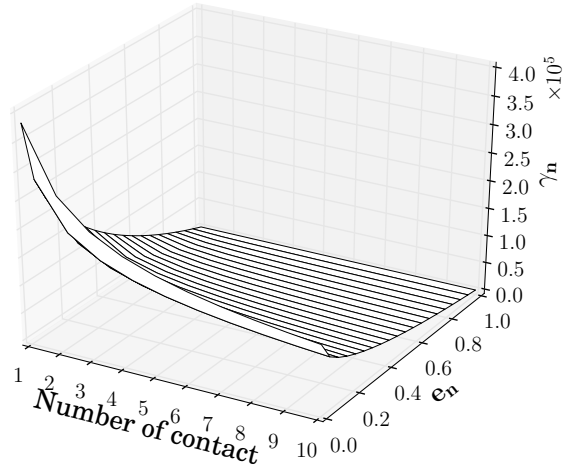
Figure 5 Dissipative normal coefficient \gamma_n as a function of restitution coefficient e_n and number of contact points N_c .
