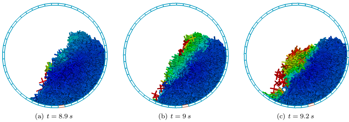
Figure 24 Avalanching regime of 2D crosses at \Omega = 5 rpm. Snapshots of the pattern of particles colored by their translational velocity magnitude (from blue (min) to red (max)) selected at 3 close times to evidence the occurrence of an avalanche.
