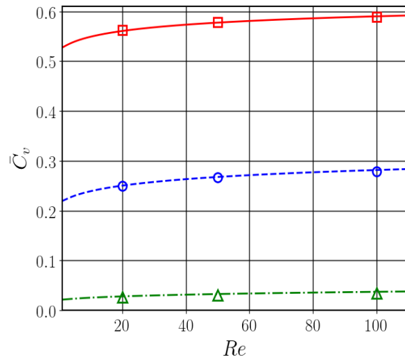
Figure 30: Steady state convection-diffusion in the flow past 3 aligned reactive spheres: mean volume concentration \overline{C}_v of sphere 3 as a function of Re in configuration A at \gamma = 0.1 and Sc = 1 . Lines correspond to model and markers correspond to numerical simulation. Red color corresponds to \phi^2 = 40 , blue color to \phi^2 = 200 and green color corresponds to \phi^2 = 4000 .
