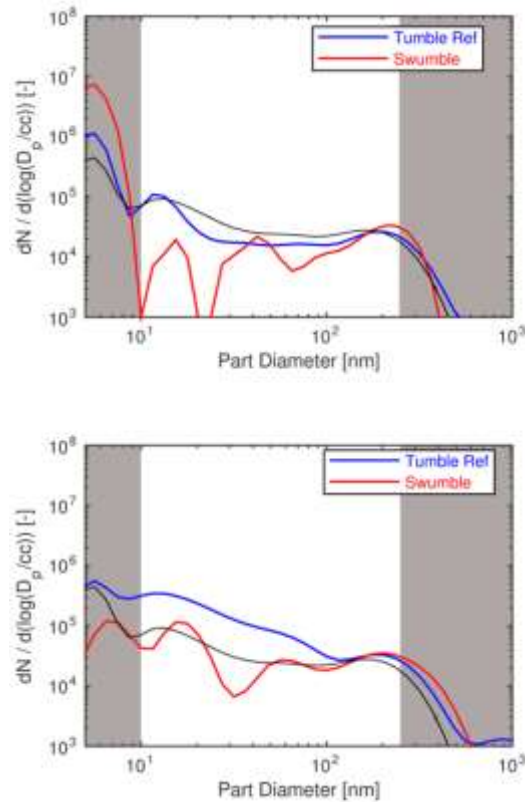
Fig. 13: Effect of in-cylinder aerodynamics on particulate emissions at two different injection phasing: SOI 260 CAD bTDC (left) and SOI 180 CAD bTDC (right). The part of the spectrum not considered for the analysis is indicated by the gray areas. The black line indicates the noise reference (PF injection case).
