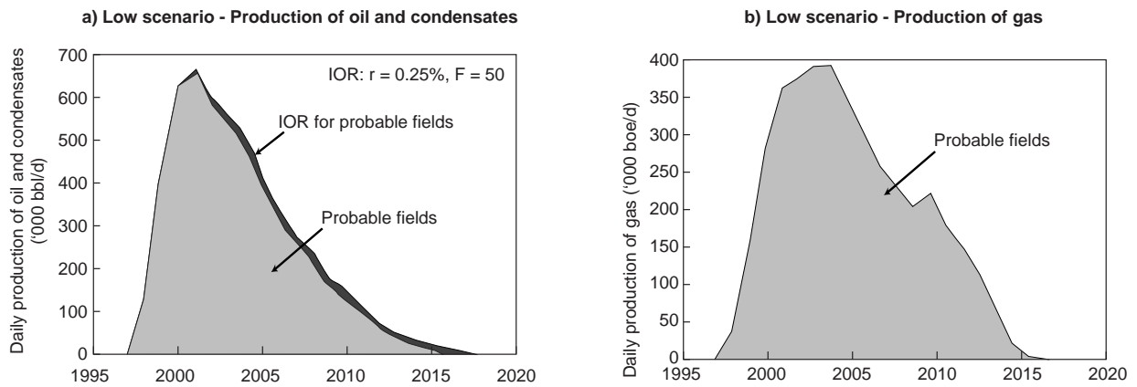
Figure 7 Low scenario – Undeveloped fields: production curves for oil, condensates and gas.
