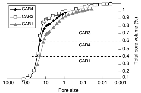
Figure 11 Mercury intrusion data.
