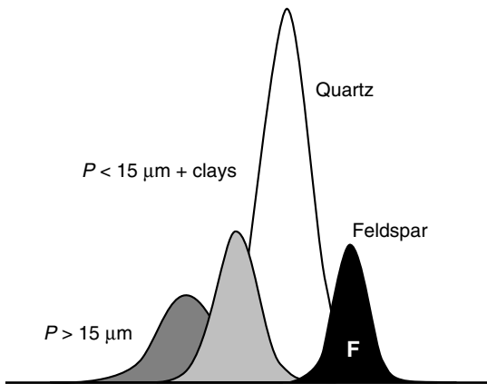
Figure 10 Grey level histogram of sample CAR4.
