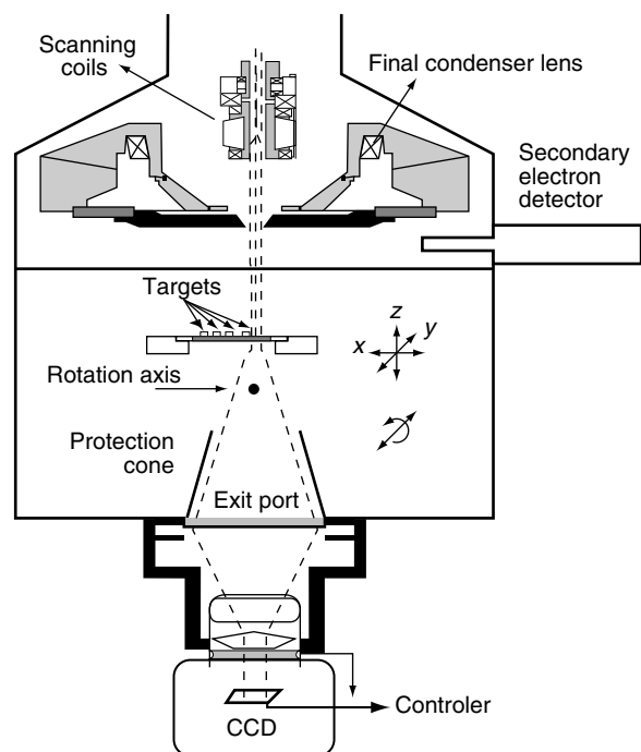
Figure 1 Schematic representation of the microtomograph.
