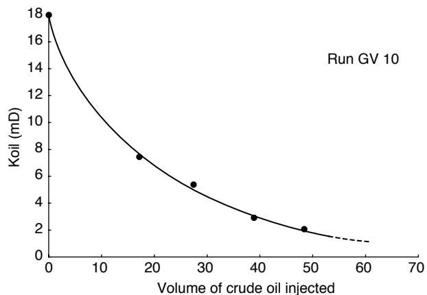
Figure 4 Oil permeability reduction in Vosges sandstone.
