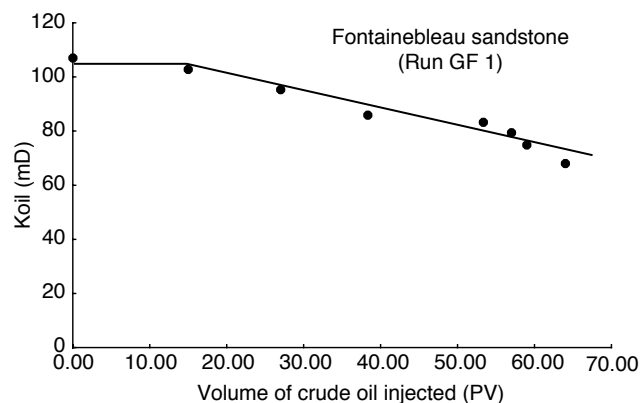
Figure 3 Oil permeability reduction in a model-porous medium.
