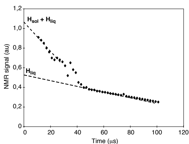
Figure 2 Relaxation curve of a mixture of liquid and solid phases.
