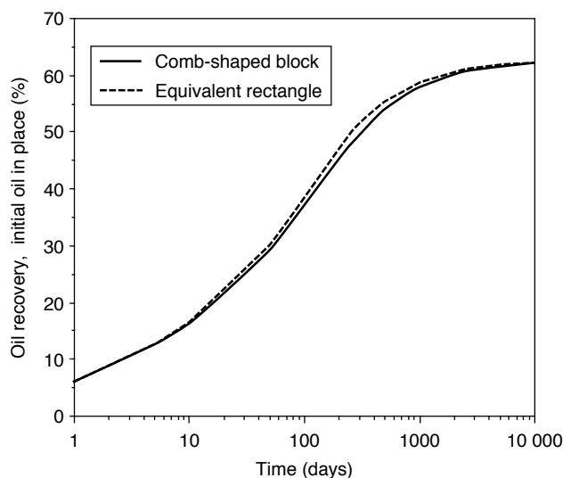
Figure 7 Water-oil imbibition in the comb-shaped block and in the equivalent rectangle.
