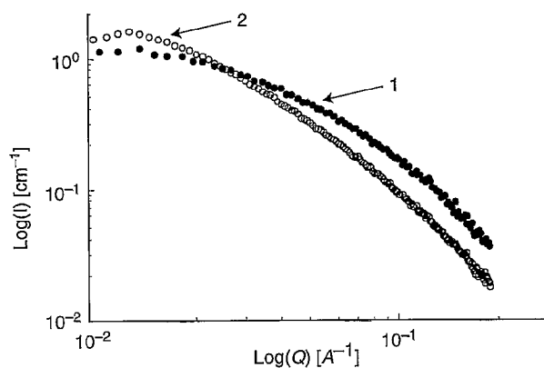
Figure 6 X-ray scattering for a mixture Safaniya vacuum residue asphaltenes (2% w/w) and resins (4% w/w) in toluene (1), and comparison with the SAXS diagram for a 2% w/w Safaniya vacuum residue asphaltene solution in toluene (2).
