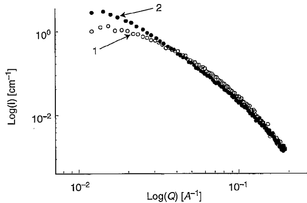
Figure 7 SAXS data for a mixture of Safaniya vacuum residue asphaltenes and resins: (1) 2% w/w asphaltene + 4% w/w resins in toluene, (2) the sum of scattering intensity for pure asphaltenes (2% w/w) and pure resins (4% w/w) in toluene.
