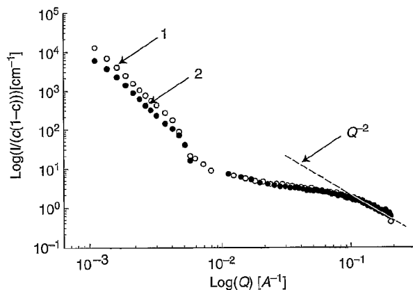
Figure 5 Small angle X-ray data for Safaniya vacuum residue resins dissolved in toluene at different concentrations c : (1) 6% w/w, (2) 10% w/w.
