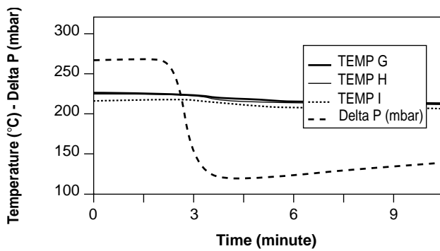
Figure 11a Stochastic regeneration 1. Temperatures inside the trap - 2000/30.
