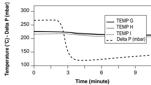
Figure 11a Stochastic regeneration 1. Temperatures inside the trap - 2000/30.
