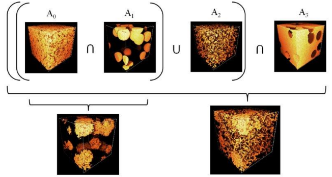
Fig. 2: Illustration of combination of Boolean models as in Table I and using Cox point process.
