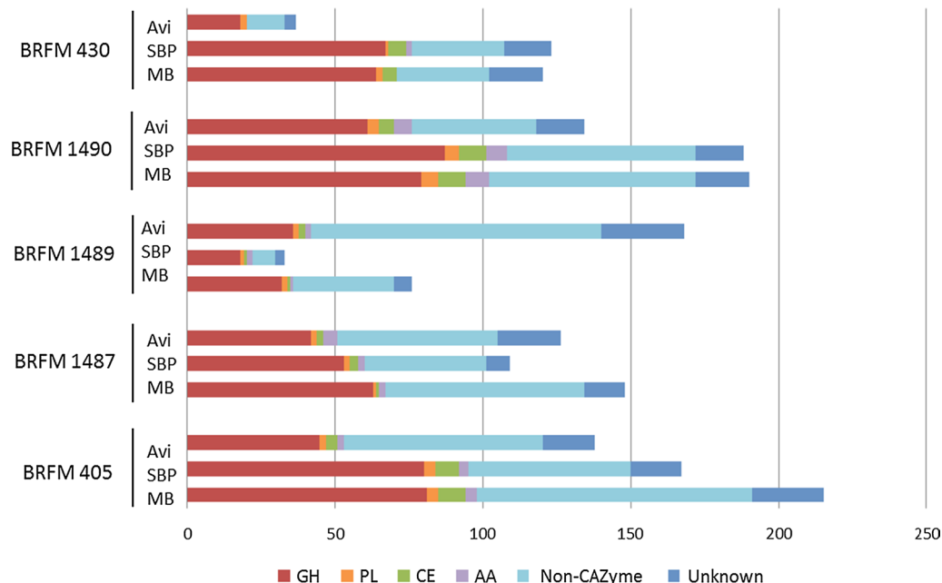
Fig. 2 Protein content of the Aspergillus spp. secretomes. Composition of the 15 secretomes in number of identified CAZymes (GH glycoside hydrolases, PL polysaccharide lyases, CE carbohydrate esterases, AA auxiliary activities), non-CAZyme proteins and proteins of unknown function
