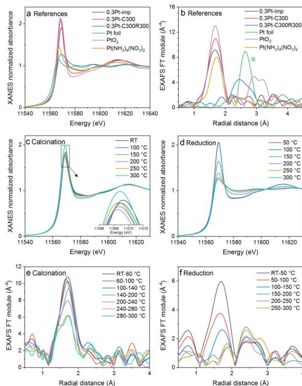
Fig. 1 XANES spectra (a) and EXAFS Fourier transform modules (b) of 0.3 wt% Pt/ \gamma -Al 2 O 3 sample, either fresh (0.3Pt-imp), or after calcination in air flow at 300 °C (0.3Pt-C300), or after subsequent reduction in H 2 flow at 300 °C (0.3Pt-C300R300), vs. standards. Evolution of XANES spectra (c,d) and EXAFS FT modules (e,f) for the 0.3Pt-imp sample during calcination in air flow (c,e) and subsequent reduction in H 2 flow (d,f) from RT to 300 °C.
