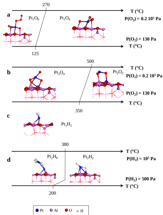
Fig. 3 Structures of the most stable oxidized (a,b) and reduced (c,d) Pt 1 and Pt 2 /γ-Al 2 O 3 (100) clusters in XAS (upper axis) and E-STEM (lower axis) conditions. Pt 1 H 2 (c) is the stable species in all reducing conditions for Pt 1 .
