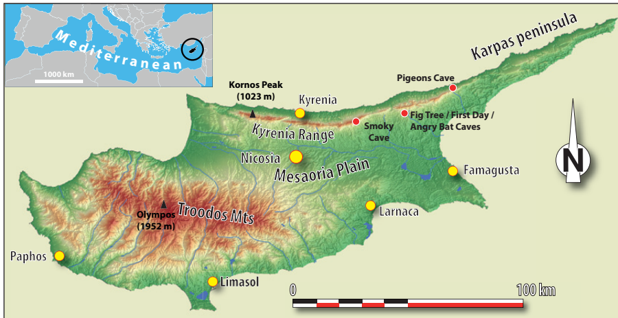
Fig. 1: Kyrenia Range is a narrow mountain range along the northern coast of Cyprus. It is made up of Carboniferous to Miocene rocks, mainly recrystallized limestones and dolostones. Troodos Mountain is made up of ophiolites surrounded by Cretaceous to Middle Miocene rocks. In-between, the Mesaoria Plain, together with the coast, are built by a layer of Miocene to recent sediments. The studied caves in Kyrenia Range are indicated by red dots.
