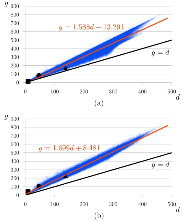
Fig. 2: Cases without skeletonization (a) and with skeletonization (b). Scatterplot of coordinates (d, g) : d (resp. g ) is the Euclidean distance (resp. geodesic distance) of a point pair. 520 locations are sampled, each pair of locations is processed. The linear regression of the scatterplot is displayed (orange line) with its equation, and the reference line g = d corresponds to geometric tortuosity equal to one. Three point pairs are represented by a black square (resp. circle and triangle).
