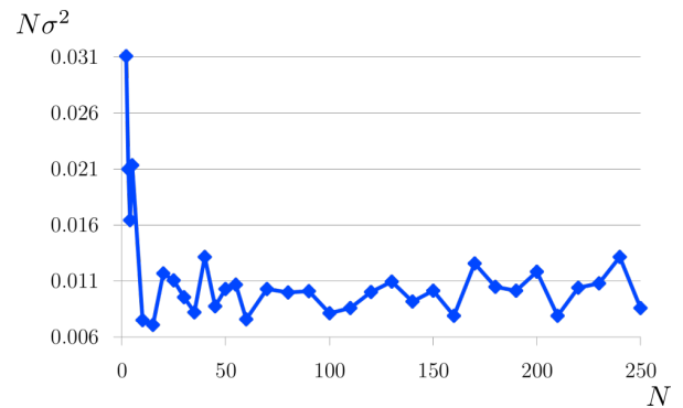
Fig. 3: Evolution of N times the variance of \hat{\tau}_M (Eq. 10), \sigma^2 , over the 100 realizations of Boolean models of size 200^3 and of volume fraction V_v = 0.7 of spheres of constant radius r = 3 , as a function of N .
