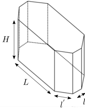
Fig. 20: The shape of a platelet grain and its parameters (Chiche et al. , 2008).
