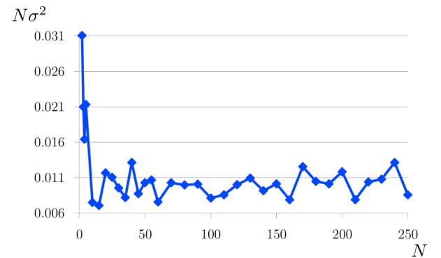
Fig. 3: Evolution of N times the variance of \hat{\tau}_M (Eq. 10), \sigma^2 , over the 100 realizations of Boolean models of size 200^3 and of volume fraction V_v = 0.7 of spheres of constant radius r = 3 , as a function of N .
