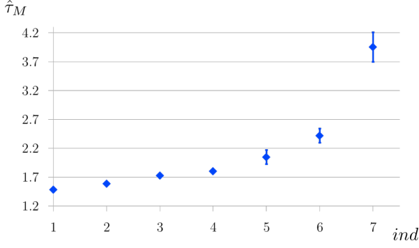
Fig. 11: \hat{\tau}_M values according to the index of (\phi_{lim,down}^2, \phi_{lim,up}^2) for the P_1 case. Confidence intervals, with confidence level at 95 % (see definition below), are represented by vertical bars.
