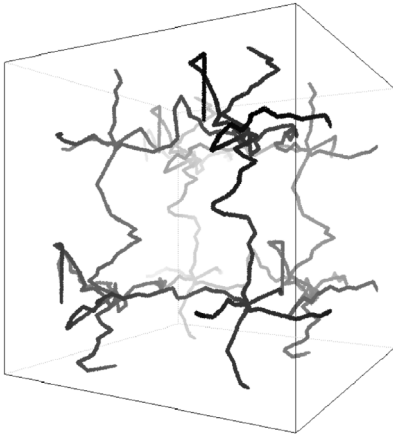
Fig. 12: Different pores with a 3D-cross structure; example of P_2 with \phi_{lim,down}^1 = \pi/8 , \phi_{lim,up}^1 = 3\pi/16 , \phi_{lim,down}^2 = 5\pi/16 and \phi_{lim,up}^2 = 3\pi/8 .
