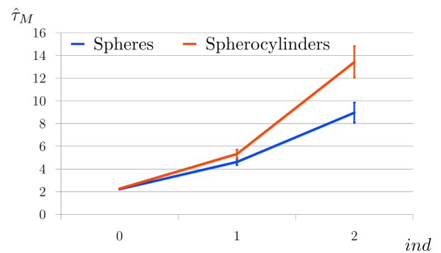
Fig. 16: M-tortuosity-by-iterative-erosions results, focus on \hat{\tau}_{M,r} , for Boolean models of spheres (blue) and spherocylinders (orange). Confidence intervals, with confidence level at 95 %, are represented by vertical bars.
