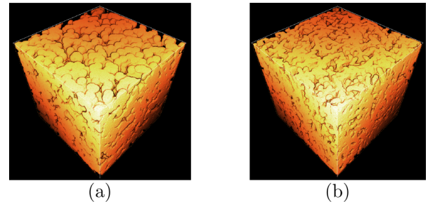
Fig. 15: Realizations of Boolean models of (a) spheres and (b) spherocylinders. Volumes generated and rendered using "plug'im!" (2018).
