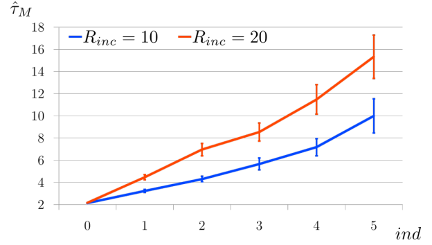
Fig. 18: The results of M-tortuosity-by-iterative-erosions , with a focus on \hat{\tau}_{M,r} , for multi-scale Cox Boolean models of spheres; R_{inc} = 10 , V_{v,inc} = 0.4 (blue), R_{inc} = 20 , V_{v,inc} = 0.6 (orange). Confidence intervals, with confidence level at 95 %, are represented by vertical bars.
