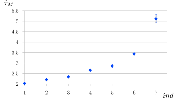
Fig. 13: \hat{\tau}_M values according to the index of (\phi_{lim,down}^2, \phi_{lim,up}^2) for the P_2 case. Confidence intervals, with confidence level at 95 % (see definition below), are represented by vertical bars.
