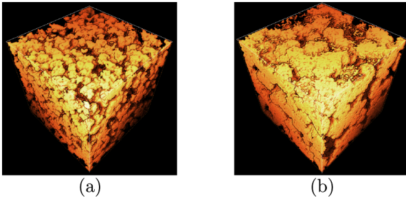
Fig. 17: Realizations of a multi-scale Cox Boolean model of spheres (a) R_{inc} = 10 , V_{v,inc} = 0.4 and (b) R_{inc} = 20 , V_{v,inc} = 0.6 . Volumes generated and rendered using "plug'im!" (2018).
