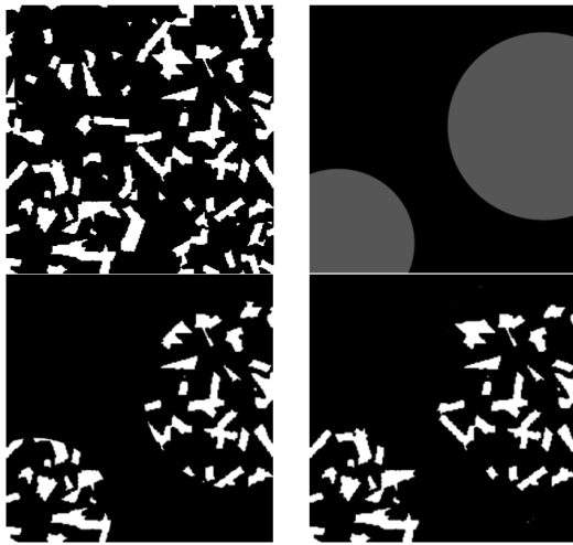
Fig. 14: Top figures: Boolean model of platelets and Boolean model of spheres denoting aggregate scale. Bottom figures: intersection of the two Boolean models, by standard operation or using Cox point process yielding a more realistic microstructure (Moreaud et al. , 2018).
