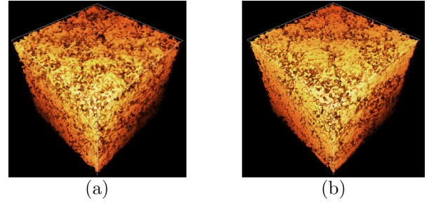
Fig. 19: Realizations of multi-scale Cox Boolean models of platelets (a) R_{inc} = 15 , V_{v,inc} = 0.3 and (b) R_{inc} = 25 , V_{v,inc} = 0.4 . Volumes generated and rendered using "plug'im!" (2018).
