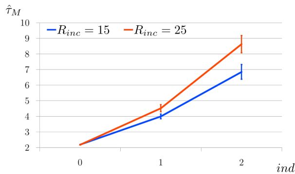
Fig. 21: M-tortuosity-by-iterative-erosions results, focus on \hat{\tau}_{M,r} , of multi-scale Cox Boolean models of platelets; R_{inc} = 15 , V_{v,inc} = 0.3 (blue), R_{inc} = 25 , V_{v,inc} = 0.4 (orange). Confidence intervals, with confidence level at 95 %, are represented by vertical bars.
