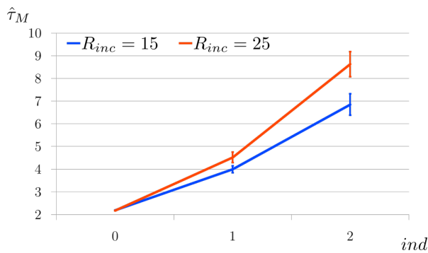
Fig. 21: M-tortuosity-by-iterative-erosions results, focus on \hat{\tau}_{M,r} , of multi-scale Cox Boolean models of platelets; R_{inc} = 15 , V_{v,inc} = 0.3 (blue), R_{inc} = 25 , V_{v,inc} = 0.4 (orange). Confidence intervals, with confidence level at 95 %, are represented by vertical bars.
