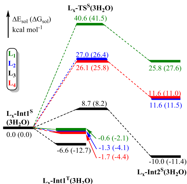
Figure 6. Reaction energy profile for O-O coupling reaction for the studied iridium catalyst series \text{Cp}^*\text{Ir-L}_{x=1-4} with three water molecules.
