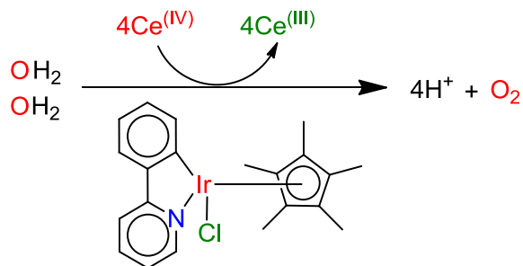
Scheme 1: Water oxidation reaction scheme using Ce(IV) as one electron donating agent for Cp*Ir-based molecular catalysts.
