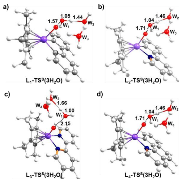
Figure 7. Transition state structures for O-O coupling reaction with three water molecules for the studied Ir catalyst series \text{Cp}^*\text{Ir-L}_{x=1-4} . Main distances are given in Å.
