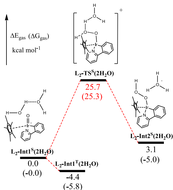
Figure 4. Reaction energy profile for O-O coupling step \text{Cp}^*\text{Ir-L}_2 catalyst with two water molecules (energies are given in \text{kcal mol}^{-1} relative to \text{L}_1\text{-Int1}^{\text{S}}(2\text{H}_2\text{O}) ).
