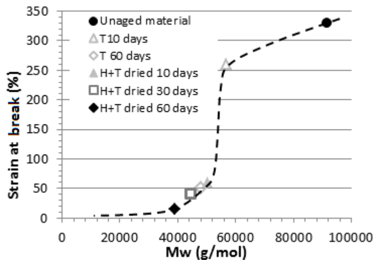
Figure 19 Strain at break as a function of weight average molar mass obtained after T ageing (110°C) and H+T ageing (pH4/110°C).
