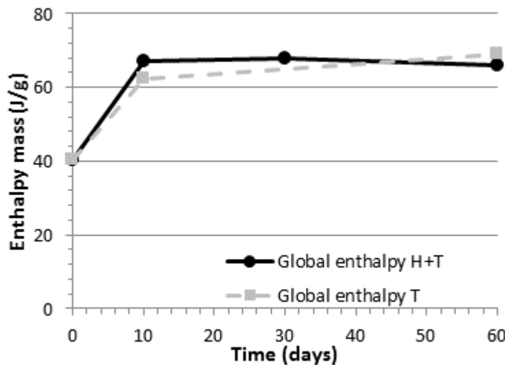
Figure 3 Total mass enthalpy for thermal (T) and thermal and hydrolyzed ageing (H+T)
