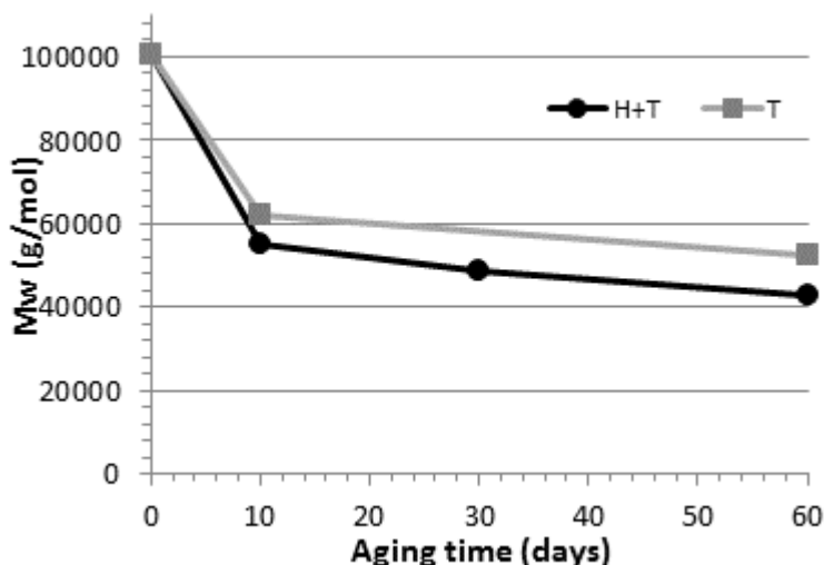
Figure 8 Decrease in molecular weight with ageing (T) and (H+T)
