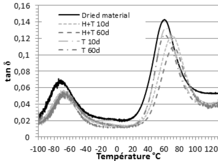
Figure 13 Evolution of tan δ before and after ageing (T) at 110° C and (H+T) at pH4 / 110°C
